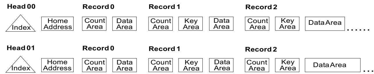
Figure 30. CKD track and record formats
