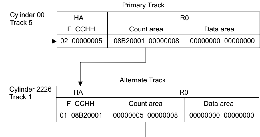
Figure 33. Primary/alternate track association (3390 model 2)
