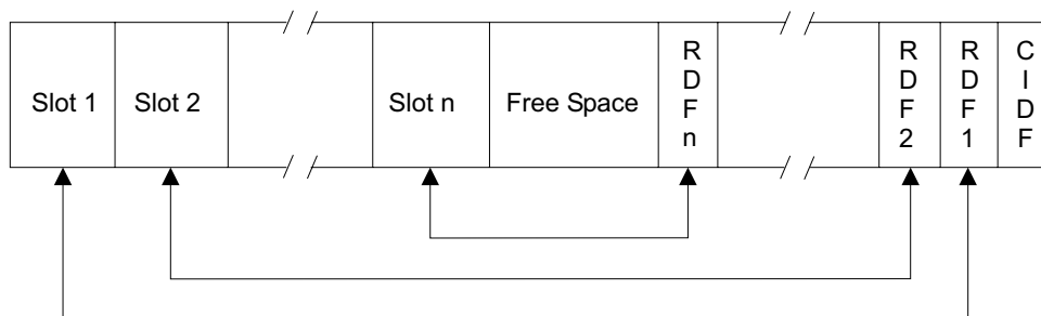
Figure 34. Format of a FBAVTOC control interval
